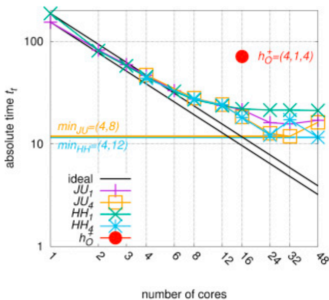
(a) Strong scaling of 100 iteration of the LBM on a single JURECA (JU) and HAZEL HEN (HH) node using the mesh with c_2 = 8.89 \cdot 10^6 cells. Furthermore, the single result at h_0^+ = (4, 1, 4) for the ODROID-MC1 is displayed. For the HPC systems the run times are shown for a single MPI rank and for four MPI ranks (indices 1 and 4).
