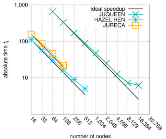
(b) Strong scalability of the LBM on the JURECA, HAZEL HEN, and JUQUEEN systems using a large production run mesh consisting of c_3 = 1.225 \cdot 10^9 cells.
